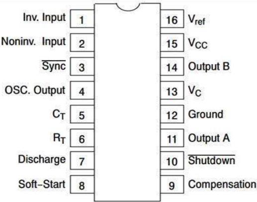
Fig.2. SG3525 pin layout
